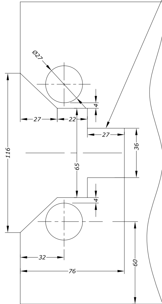
DETAIL AT 'Y'
