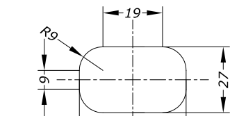
DETAIL AT 'D'
